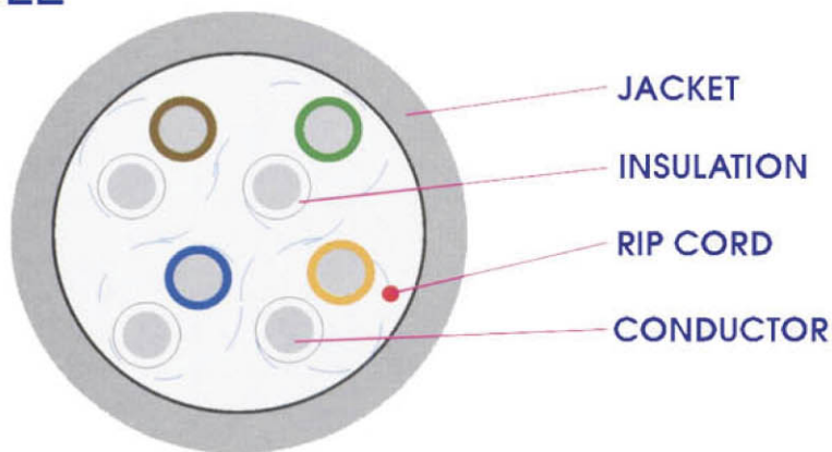
UTP CAT 5e 4P Cross-Section Structure
